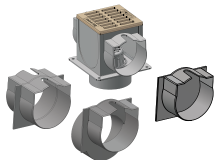
Universal Fitting Kit can be assembled into an Elbow, Tee, Cross, Coupling, or End Cap. All configurations available with or without bottom outlet.
