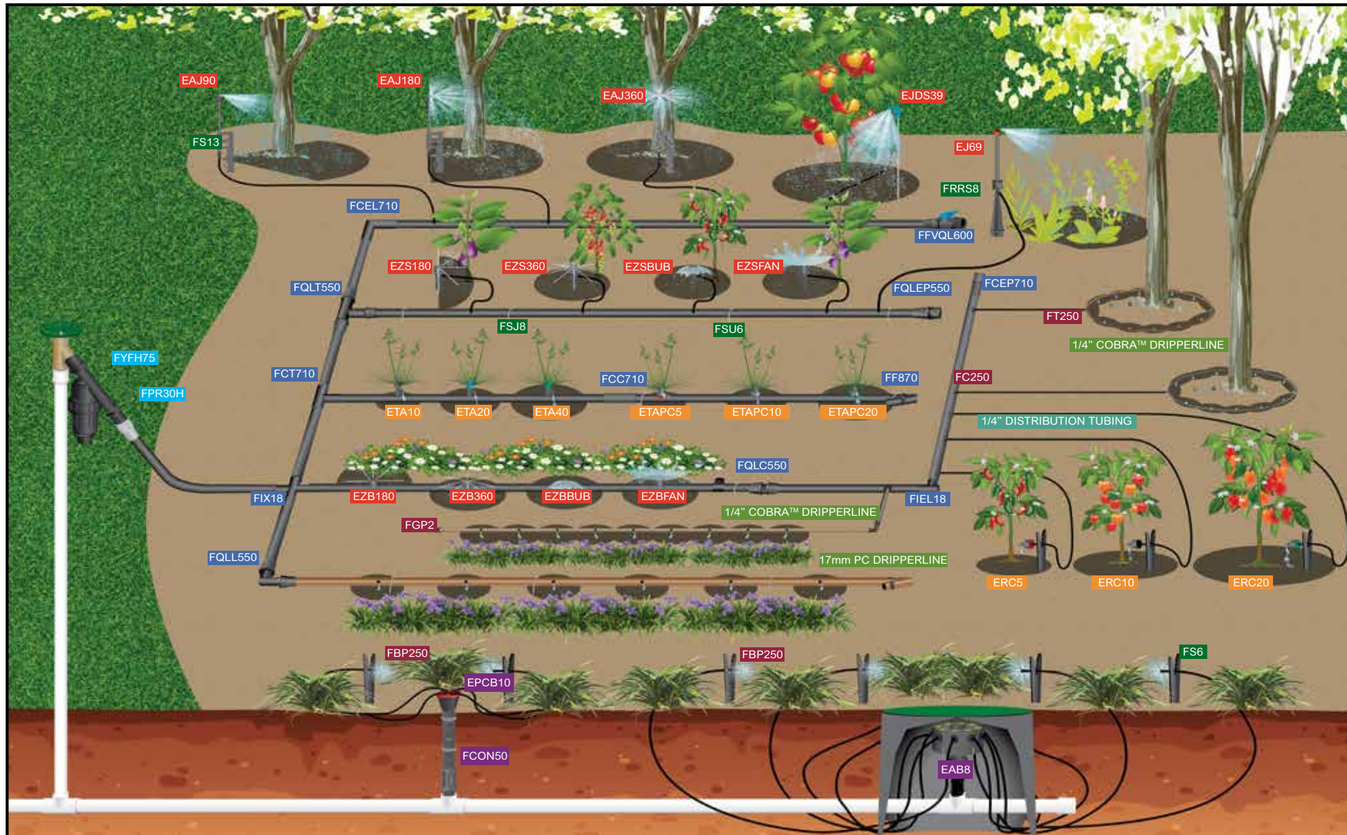
1/4" POLY OR VINYL DISTRIBUTION TUBING 1/2" POLY SUPPLY TUBING
