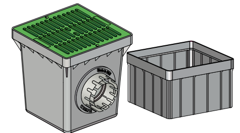
9", 12", or 18" Catch Basins with 2 or 4 Outlets 9", 12" and 18" Risers Available
